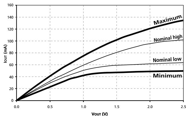
Figure 9: Pull-Up Characteristics
