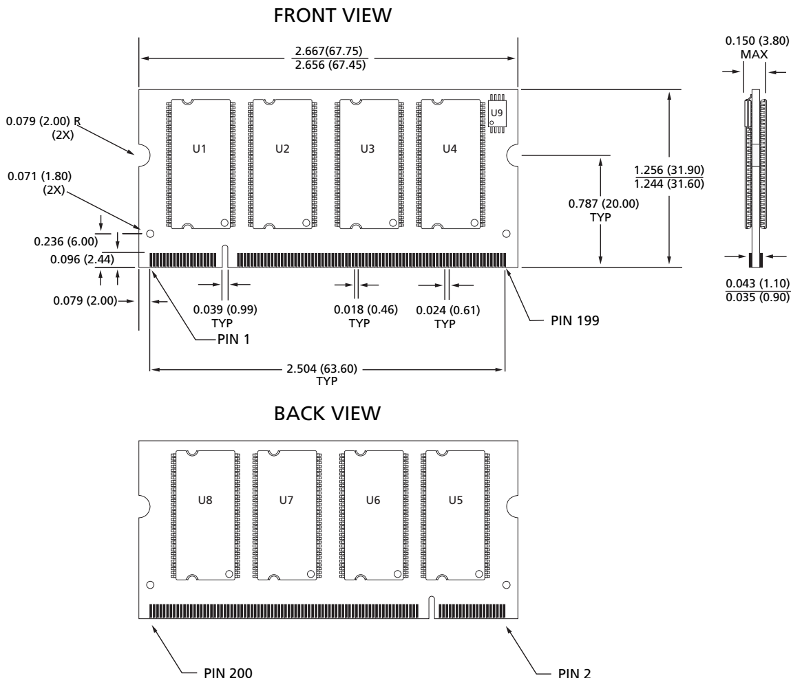
Figure 15: 200-Pin DDR SODIMM Dimensions
