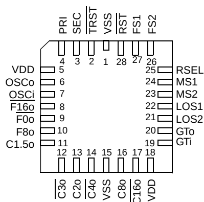
Figure 2 - Pin Connections
