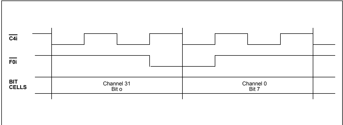
Figure 9 - Frame Alignment
