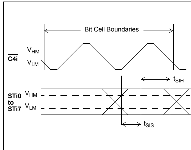
Figure 13 - Serial Inputs
