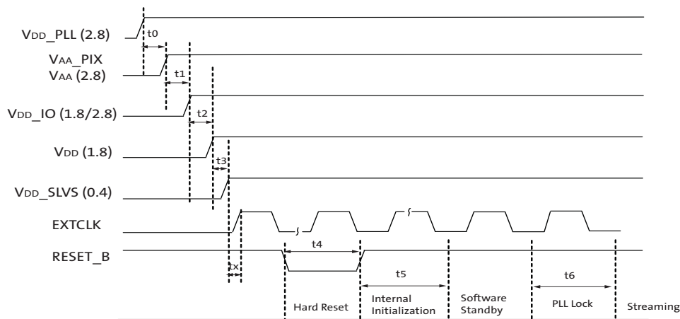
Figure 11: Power Up
