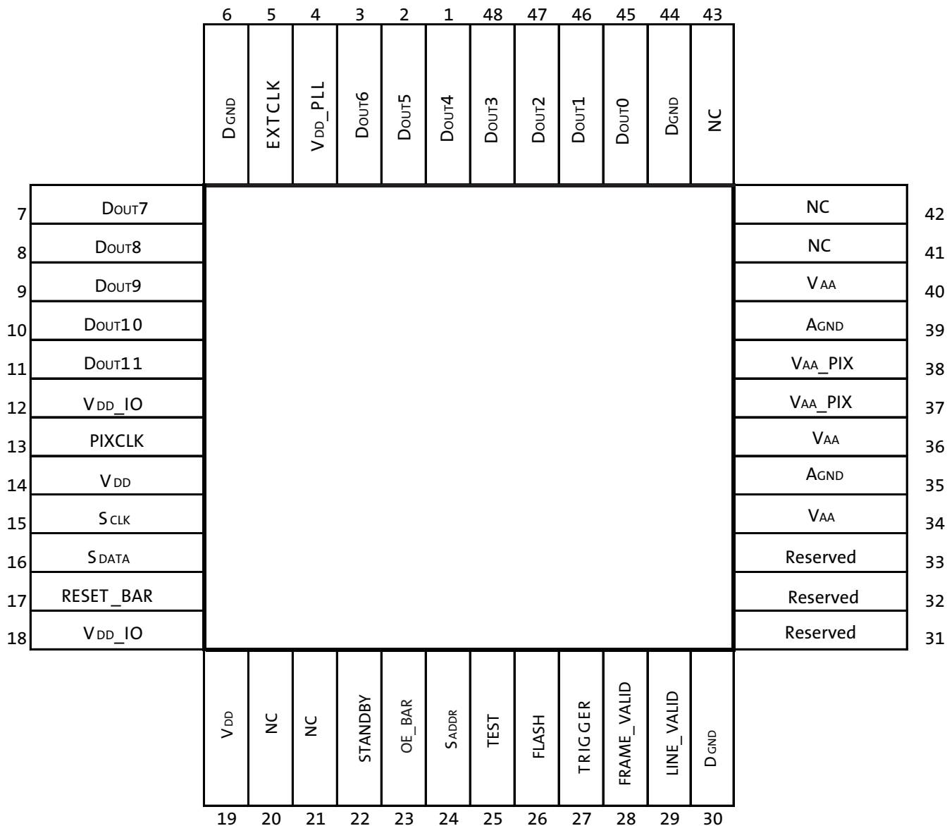
Figure 5: 48 iLCC Package, Parallel Output
