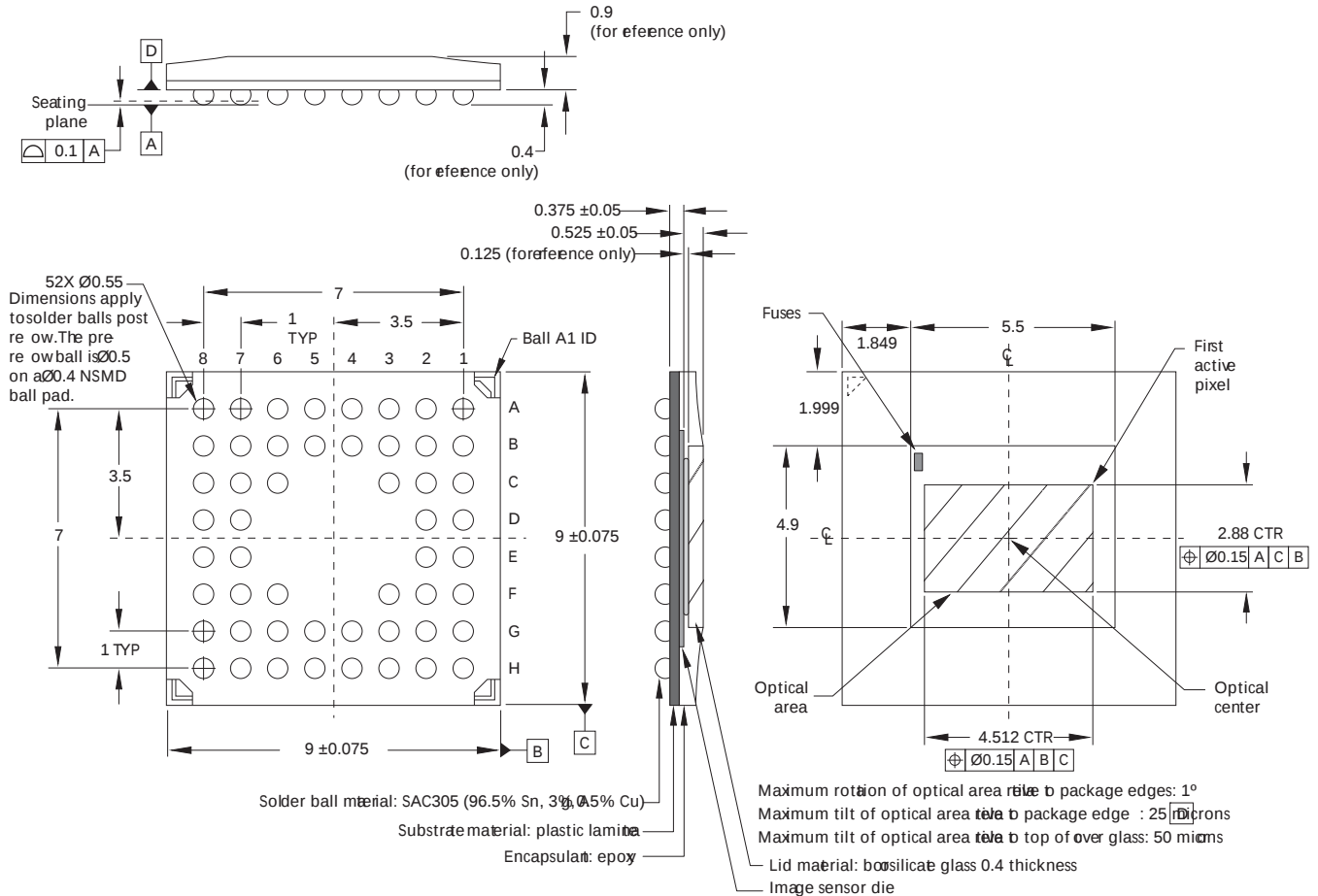
Figure 47: 52-Ball IBGA
