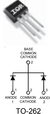
MURB2020CT-1PbF
