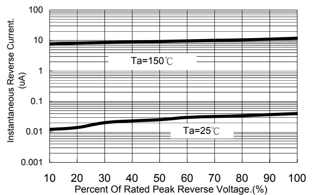
Fig. 6 Typical Reverse Characteristics (MURS340S~360S)
