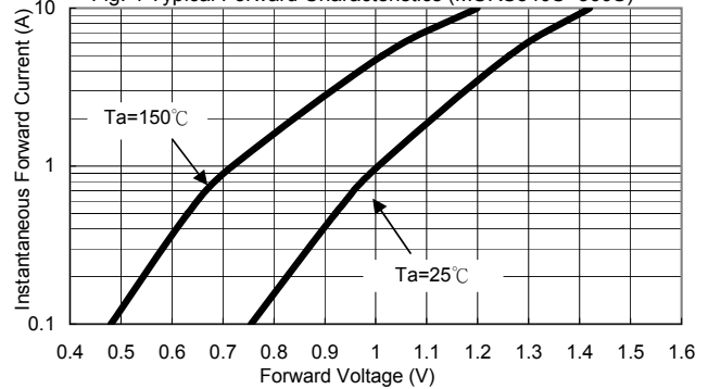
Fig. 4 Typical Forward Characteristics (MURS340S~360S)
