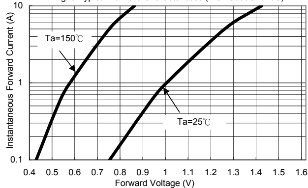
Fig. 3 Typical Forward Characteristics (MURS305S~320S)
