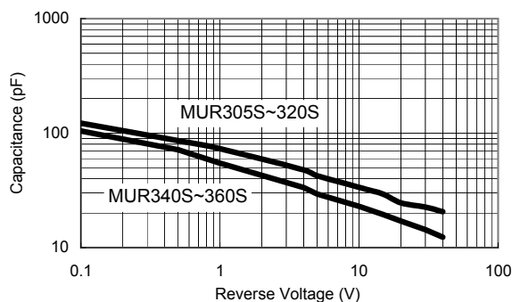
Fig. 7 Typical Junction Capacitance
