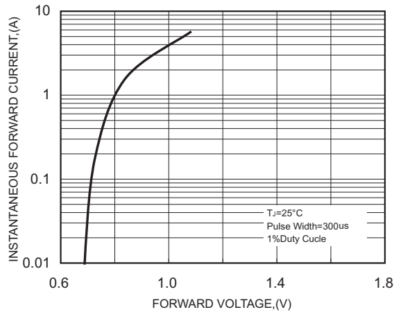
FIG.1-TYPICAL FORWARD CHARACTERISTICS
