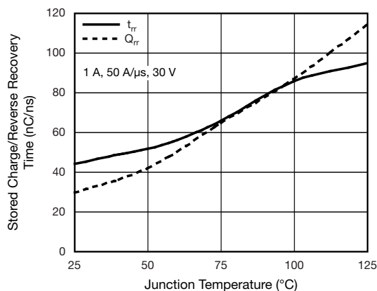
Fig. 5 - Typical Reverse Switching Characteristics
