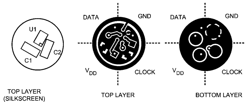
FIGURE 12. PCB Layout
