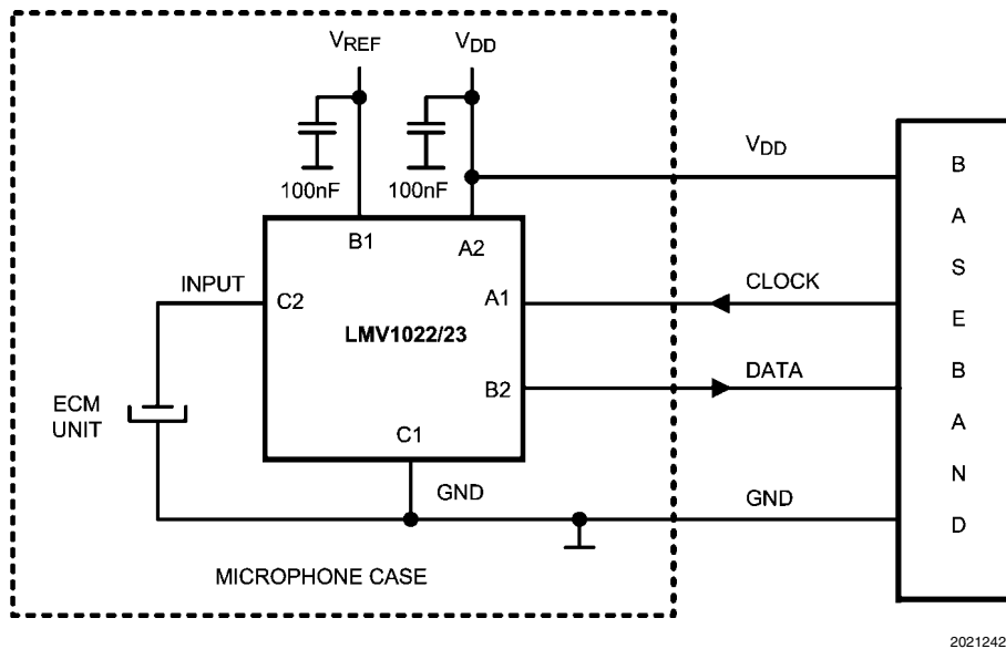
FIGURE 1. Typical Application
