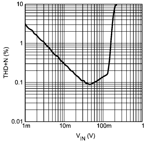
THD vs. Input Level at 16kbit/s, CLOCK Frequency = 0.8MHz
