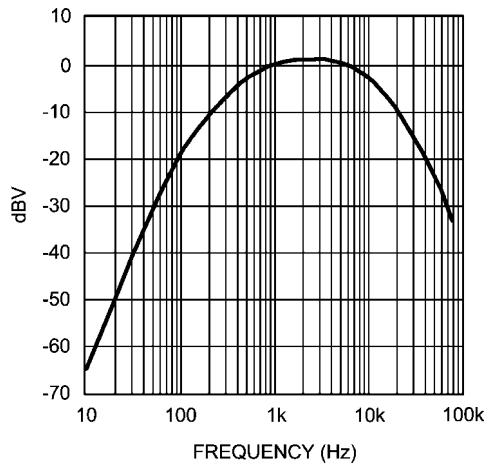
FIGURE 4. A-weighted Filter
