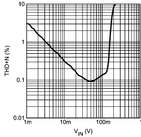
THD vs. Input Level at 24kbit/s, CLOCK Frequency = 1.6MHz
