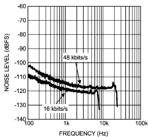
Output Noise Spectrum at 16kbit/s and 48kbit/s
