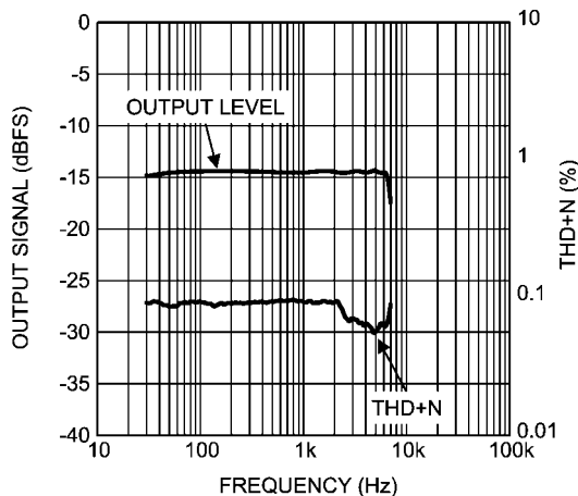
THD and Output Level vs. Frequency at 16bBit/s, CLOCK Frequency = 0.8MHz V_{in} = 50\text{mV}_{pp}
