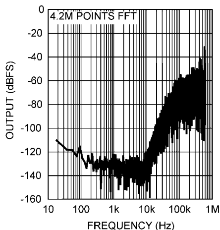
FIGURE 7. Frequency Spectrum
