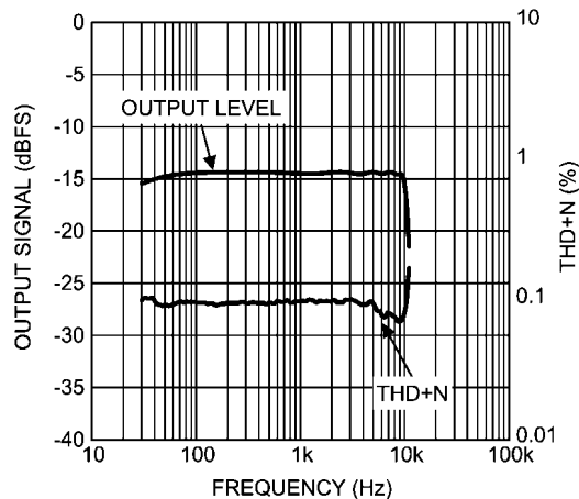
THD and Output Level vs. Frequency at 24kbit/s, CLOCK Frequency = 1.2MHz V_{in} = 50\text{mV}_{pp}
