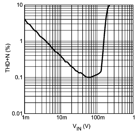
THD vs. Input Level at 48kbit/s, CLOCK Frequency = 2.4MHz
