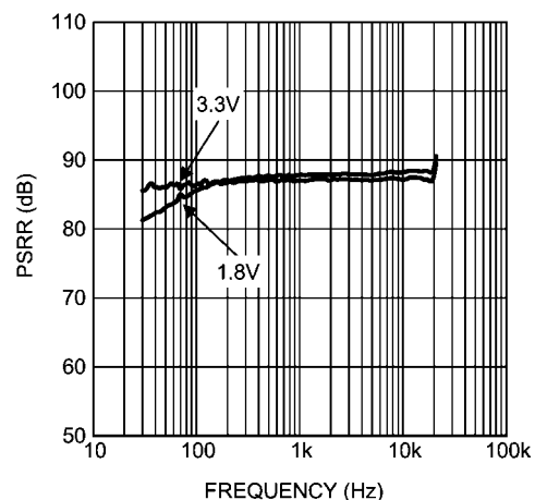
PSRR vs. Frequency for V_{DD} = 1.8V and 3.3V at 48kbit/s, CLOCK Frequency = 2.4MHz
