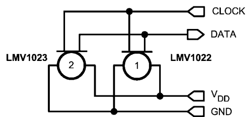
FIGURE 9. Stereo Application
