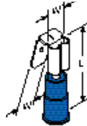
MVU14-250DM 16-14 0.250 Male/Female
