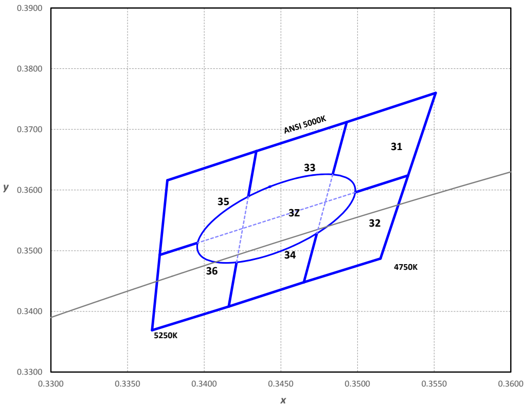
Figure 19. ANSI 5000K 1/7 th color bin structure.
