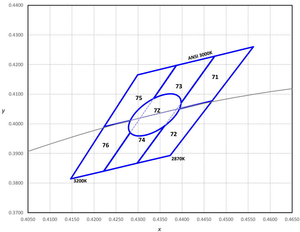
Figure 16. ANSI 3000K 1/7 th color bin structure.
