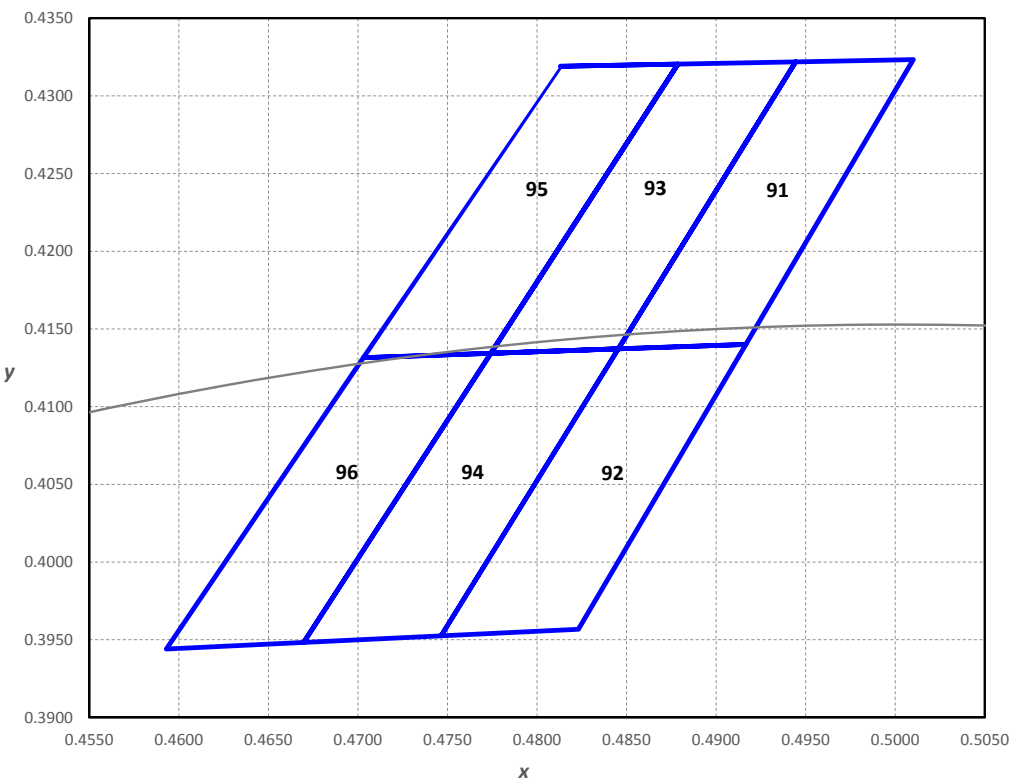
Figure 14. 2500K 1/6 th ANSI color bin structure.
