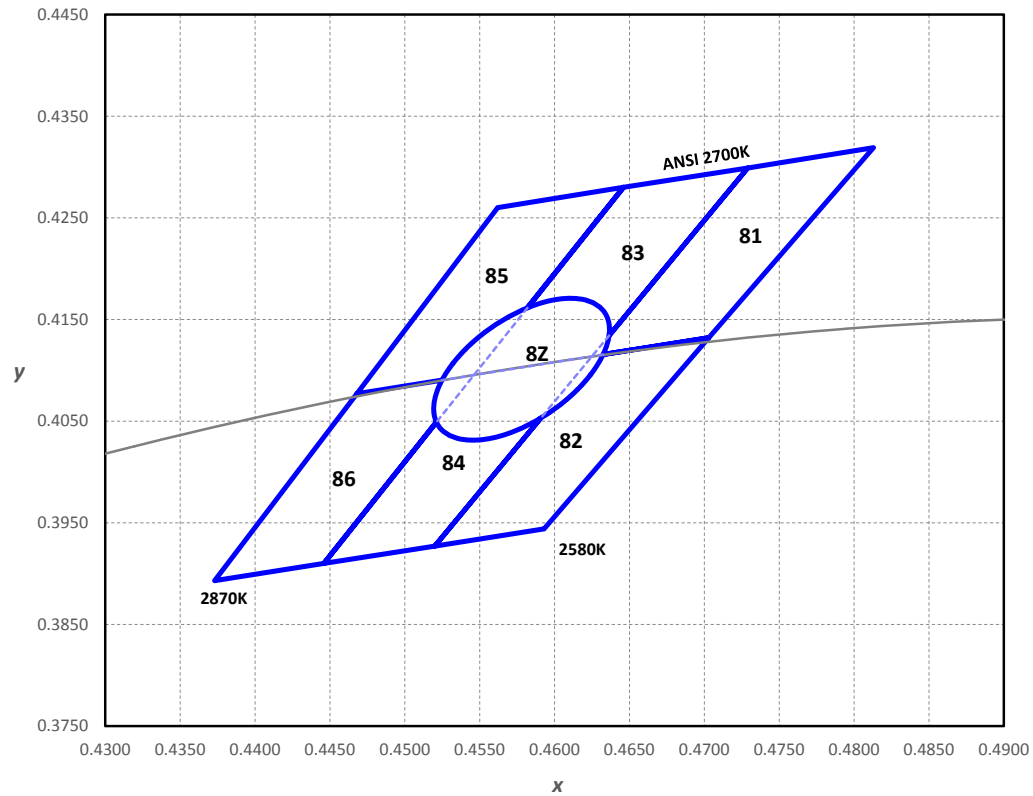
Figure 15. ANSI 2700K 1/7 th color bin structure.
