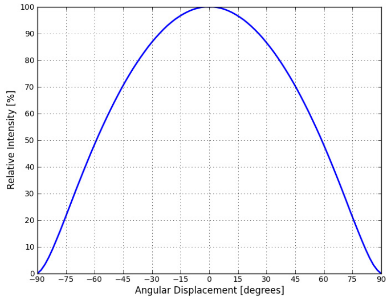
Figure 9. Typical representative spatial radiation pattern.
