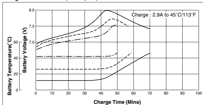
Charge Characteristics (5 cells pack)
