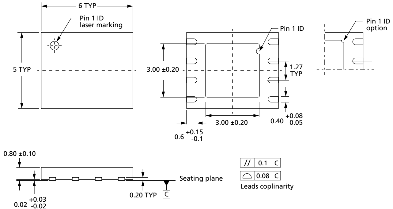
Figure 40: V-PDFN-8 6mm x 5mm (MLP8) – Package Code: F6
