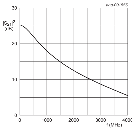
T_{amb} = 25 °C; I_{CC(tot)} = 6 mA; V_{CC} = 3 V; P_i = -30 dBm.
