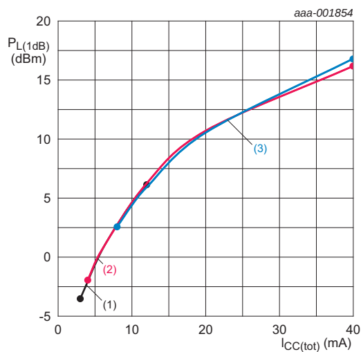
T_{amb} = 25 °C; f = 900 MHz. (1) V_{CC} = 1.5 V (2) V_{CC} = 3 V (3) V_{CC} = 5 V
