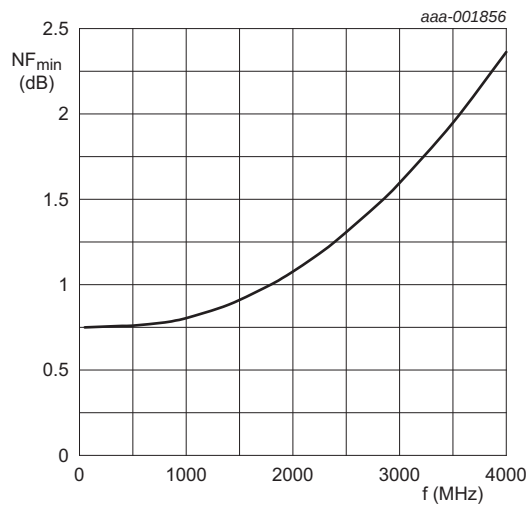
T_{amb} = 25 °C; I_{CC(tot)} = 6 mA; V_{CC} = 3 V.
