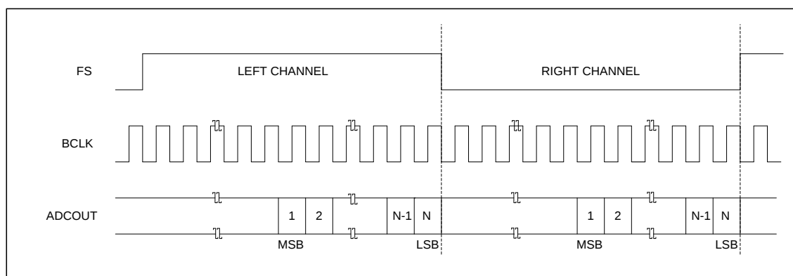
Figure 32: Right Justified Audio Interface (Special mode)
