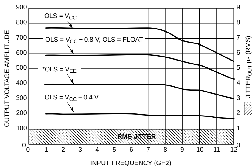
Figure 5. Output Voltage Amplitude (V OUTPP ) / RMS Jitter vs. Input Frequency (f in ) for DFF Mode (V CC - V EE = 2.5 V @ 25°C; Repetitive 1010 Input Data Pattern)
