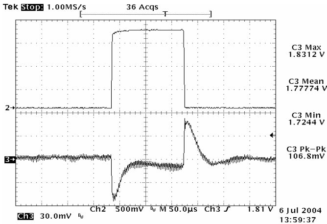
Figure 21: Typical transient response to step load change at 10A/μs from 50% to 75% and 75% to 50% of I_o , max at 12Vin, 1.8V out
