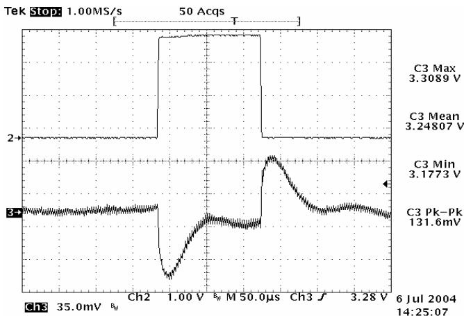
Figure 23: Typical transient response to step load change at 10A/μs from 50% to 75% and 75% to 50% of I_o , max at 12Vin, 3.3V out
