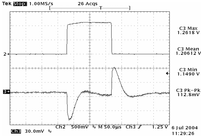
Figure 19: Typical transient response to step load change at 10A/μs from 50% to 75% and 75% to 50% of I_o , max at 12Vin, 1.2V out
