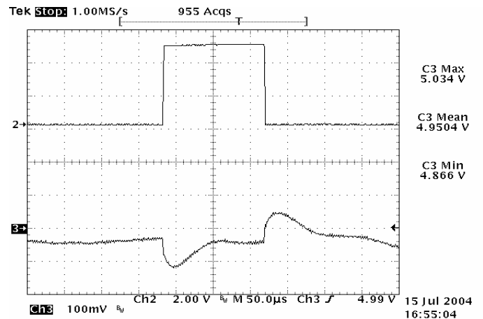
Figure 24: Typical transient response to step load change at 10A/μs from 50% to 75% and 75% to 50% of I_o , max at 12Vin, 5.0V out
