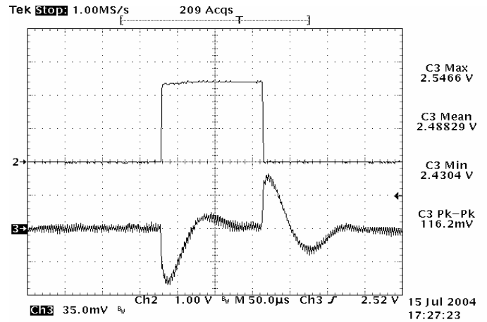
Figure 22: Typical transient response to step load change at 10A/μs from 50% to 75% and 75% to 50% of I_o , max at 12Vin, 2.5V out
