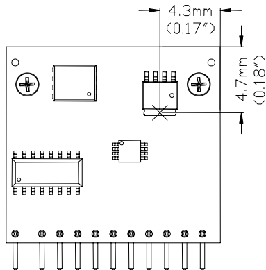
Figure 33: Temperature measurement location * The allowed maximum hot spot temperature is defined at 130 °C
