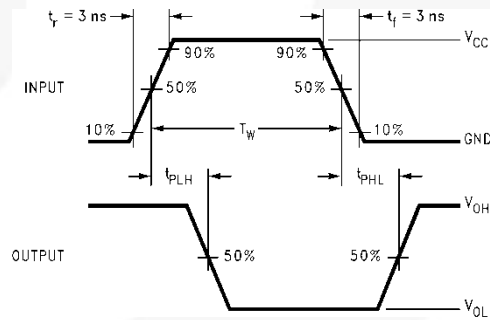
Figure 6. AC Waveforms
