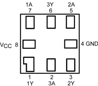
Figure 4. MicroPak™ (Top Through View)
