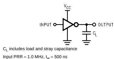
FIGURE 1. AC Test Circuit
