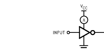
FIGURE 2. I CCD Test Circuit
