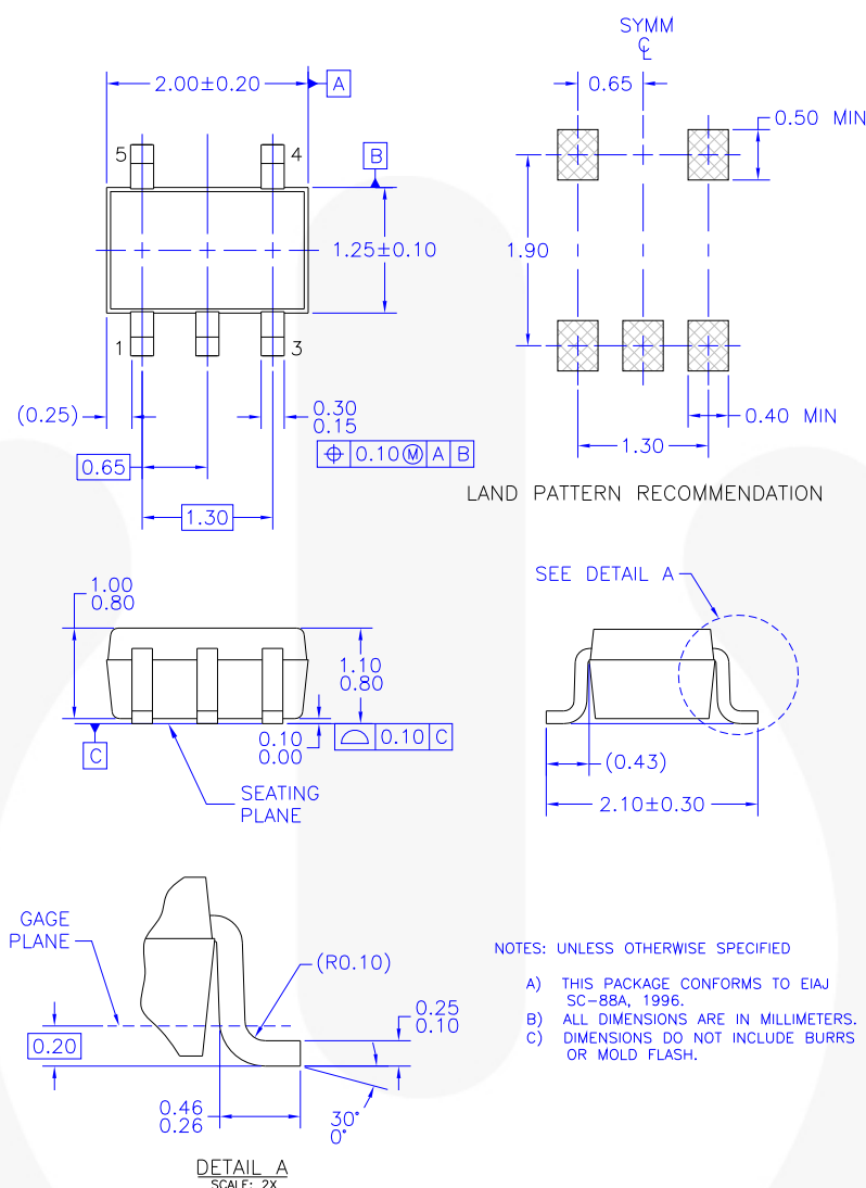
Figure 7. 5-Lead, SC70, EIAJ SC-88a, 1.25mm Wide
