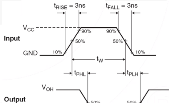
Figure 6. AC Waveforms
