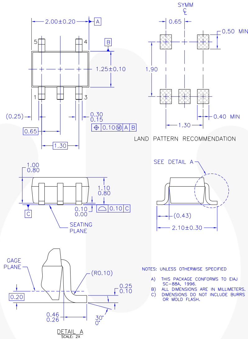
Figure 8. 5-Lead, SC70, EIAJ SC-88a, 1.25mm Wide
