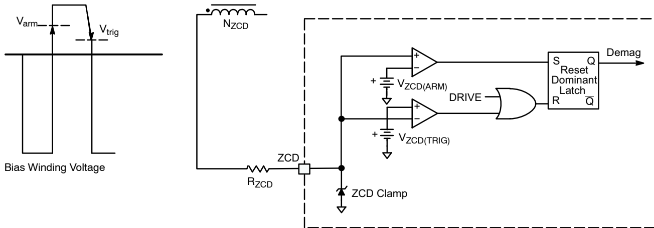
Figure 27. ZCD Operation
