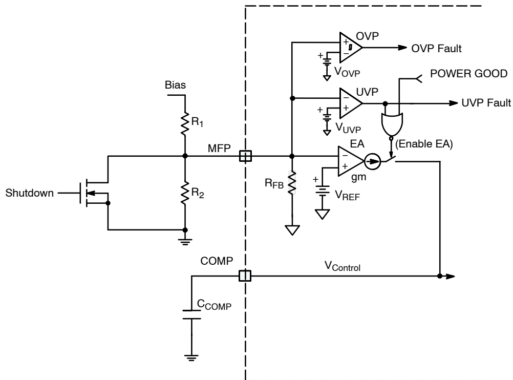
Figure 29. Multi-Function Pin Operation
