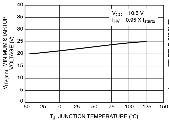
Figure 8. Minimum Startup Voltage vs. Junction Temperature
