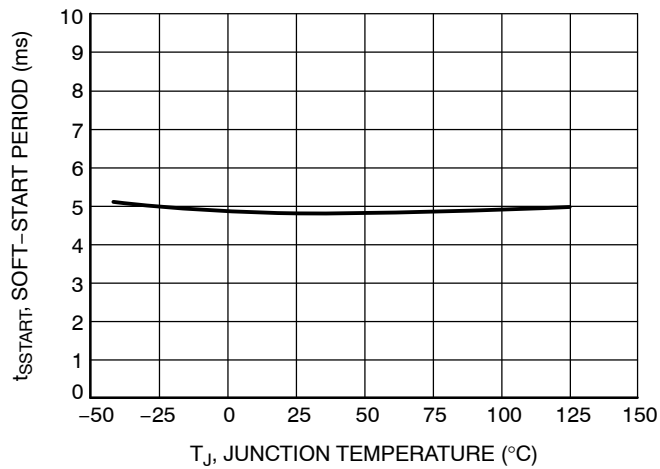
Figure 23. Soft-Start Period vs. Junction Temperature
