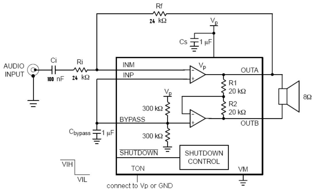
Figure 4. Single-ended Configuration
