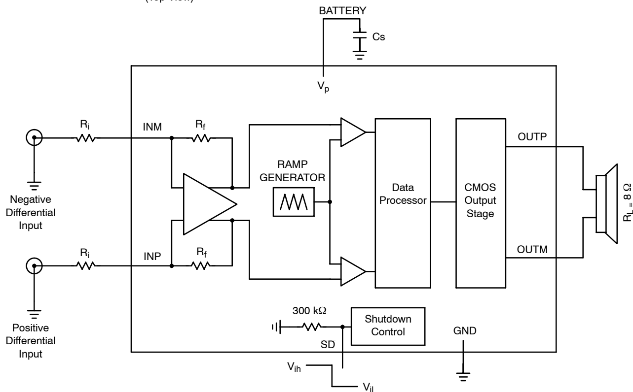
Figure 1. Typical Application
