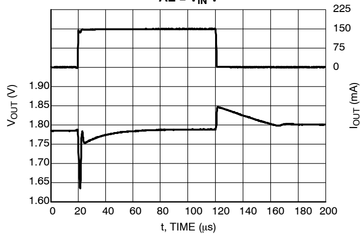
Figure 63. Load Transients, 1.8 V Version, I_{OUT} = 1 - 150 \text{ mA} , t_R = t_F = 0.5 \mu s , V_{IN} = 2.8 \text{ V} , AE = 0 \text{ V}
