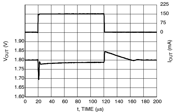
Figure 64. Load Transients, 1.8 V Version, I_{OUT} = 1 - 150 \text{ mA} , t_R = t_F = 0.5 \mu s , V_{IN} = 2.8 \text{ V} , AE = V_{IN} \text{ V}
