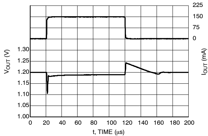
Figure 62. Load Transients, 1.2 V Version, I_{OUT} = 1 - 150 \text{ mA} , t_R = t_F = 0.5 \mu s , V_{IN} = 2.2 \text{ V} , AE = V_{IN} \text{ V}
