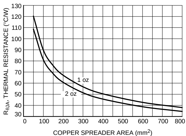
Figure 22. R_{\theta JA} vs. Copper Spreader Area, D²PAK 3-Lead
