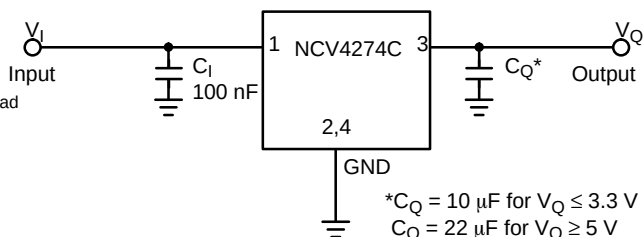
Figure 3. Application Circuit
