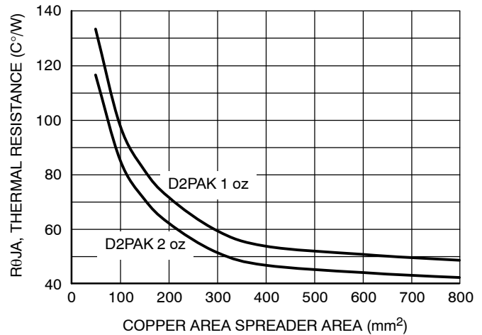
Figure 25. \theta_{JA} vs. Copper Spreader Area, D2PAK 5-Lead
