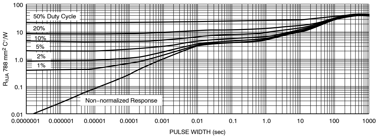
Figure 29. Duty Cycle for 1" Spreaders Boards, D²PAK 5-Lead
