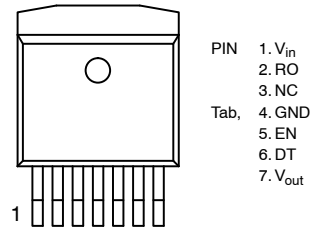
D 2 PAK-7
