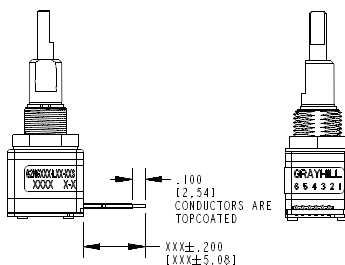
.050" Stripped Cable
