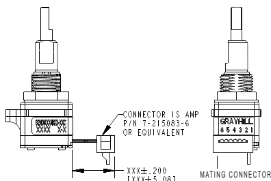
.050" Connector
