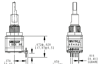
.050" Pin Header
