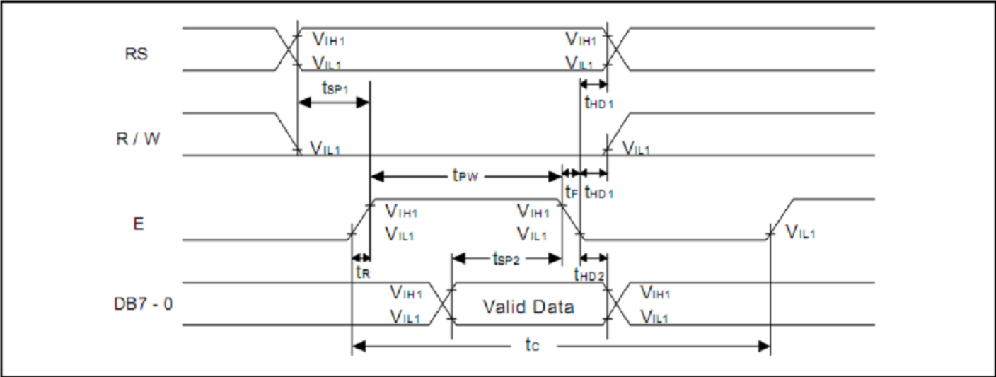
Write mode timing diagram (Writing data from MPU to S6A0069)
