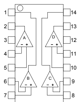
NJM12901M
