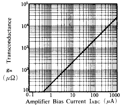
Transconductance
