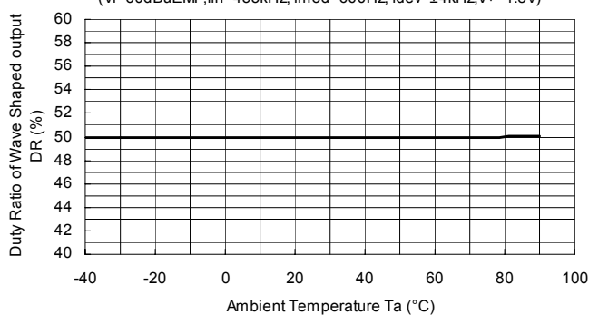
Duty Ratio of Wave Shaped Output versus Ambient Temperature
