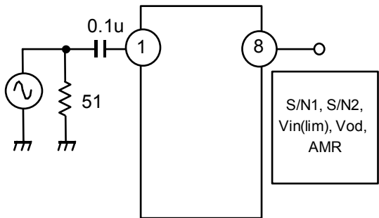
Test Circuit 1 S/N1, S/N2, Vin(lim), Vod, AMR
