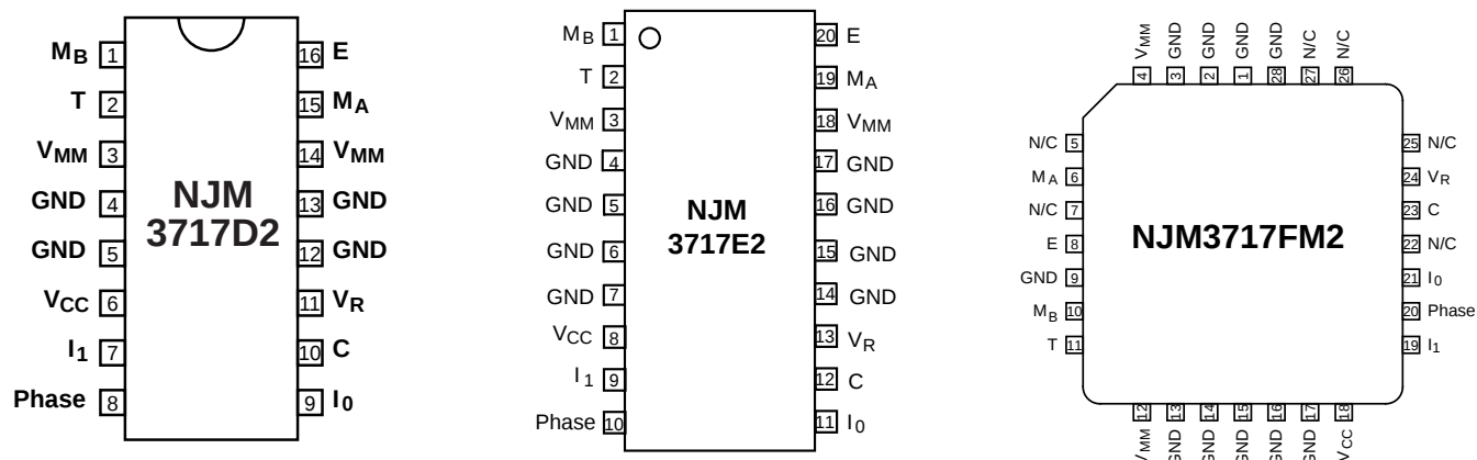
Figure 2. Pin configurations
