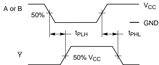
Figure 5. Switching Waveform
