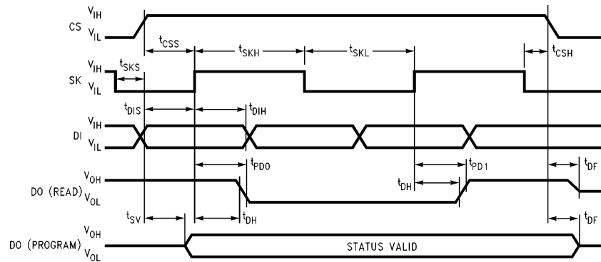
Synchronous Data Timing
