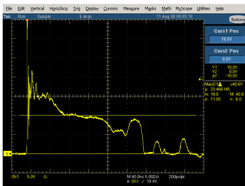
Figure 1. ESD Clamping Voltage Screenshot (8 kV Contact per IEC61000-4-2)
