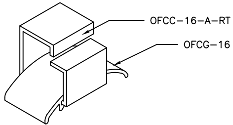
TYPICAL ASSEMBLY
