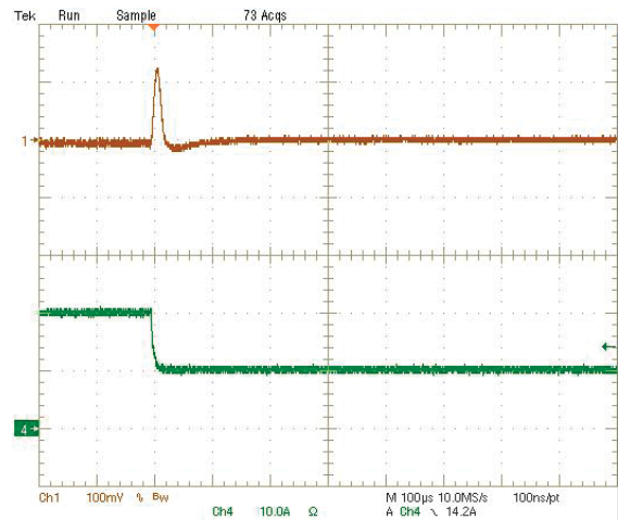
Step Load Transient Response (Vin=12V, Vout=1.8V, Cload=188μF, Iout=20A to 10A) Trace 1=Vout, 100 mV/div(AC), Trace 4=Iout, 10A/div.
