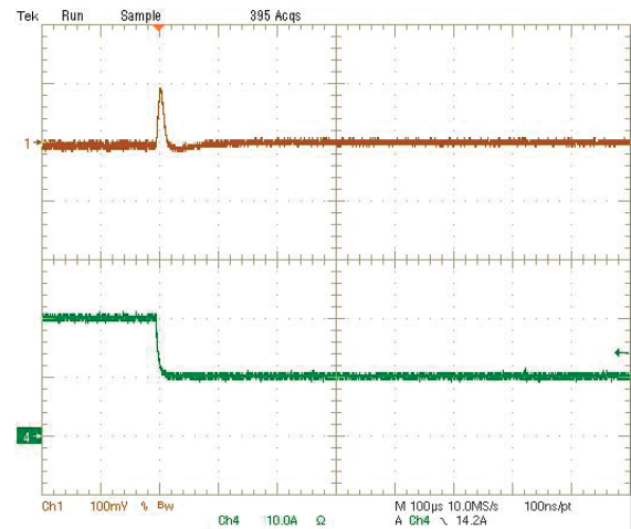
Step Load Transient Response (Vin=12V, Vout=2.5V, Cloud=188μF, Iout=20A to 10A) Trace 1=Vout, 100 mV/div(AC), Trace 4=Iout, 10A/div.
