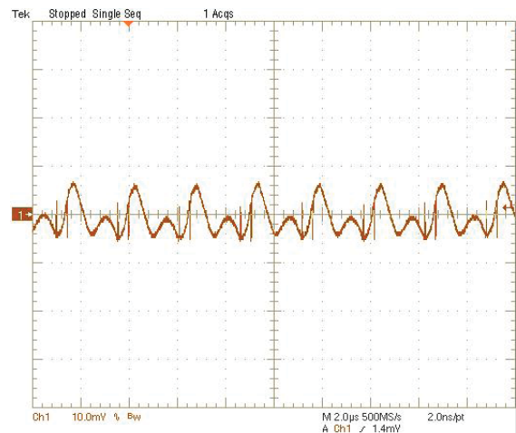
Output Ripple and Noise (Vin=12V, Vout=1.8V, Iout=20A, Cload=188μF, ScopeBW=20MHz) Trace1=Vout, 10mV/div(AC)
