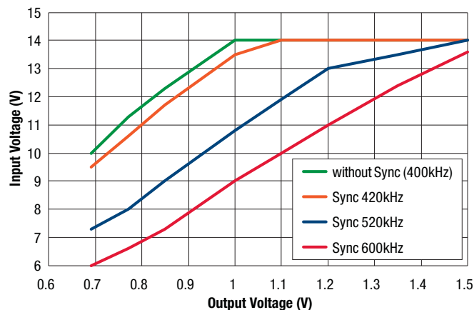
Figure 9 Voltage Range Graph (range expansion)
