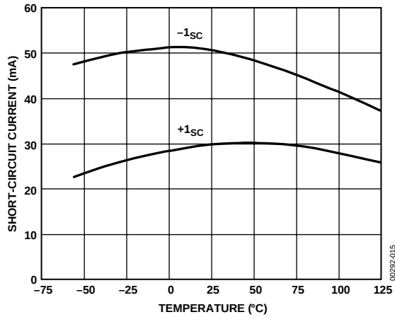
Figure 15. Short-Circuit Current vs. Temperature @ \pm 15 V
