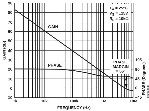
Figure 20. Open-Loop Gain and Phase vs. Frequency @ \pm 15 V
