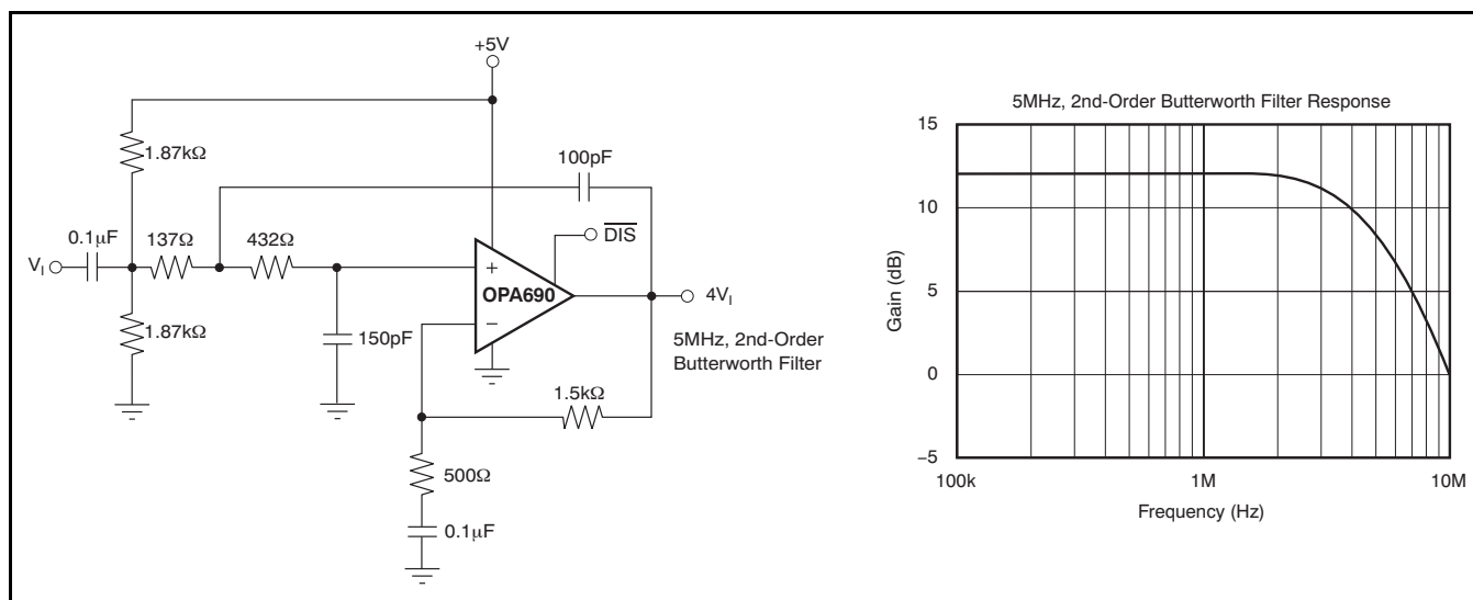
Figure 42. Single-Supply, High-Frequency Active Filter
