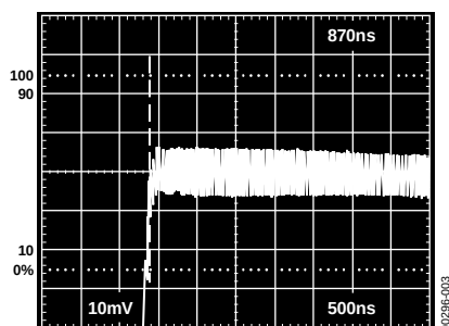
Figure 3. Fast Settling (0.01%)
