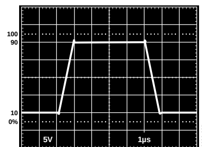
Figure 5. Excellent Output Drive, R_L = 600\text{ }\Omega
