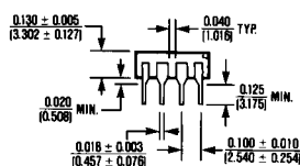
8 Lead Plastic DIP \theta_{JA} = 120^{\circ}\text{C/W} \theta_{JC} = 70^{\circ}\text{C/W}
