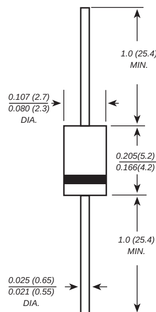
DO-41
