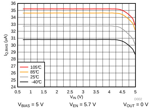
Figure 4. I_{Q,BIAS} vs V_{IN}
