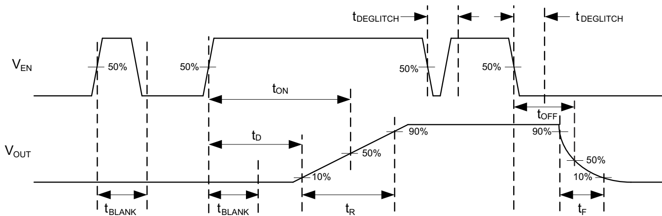
Figure 2. Timing Waveforms
