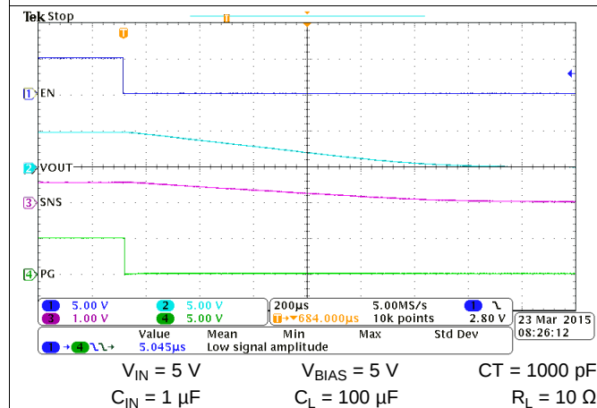
Figure 48. PG Response to EN Falling ( t_{DEGLITCH} )
