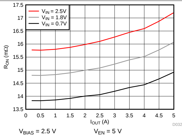
Figure 15. R_{ON} vs I_{OUT} , V_{BIAS} = 2.5\text{ V}
