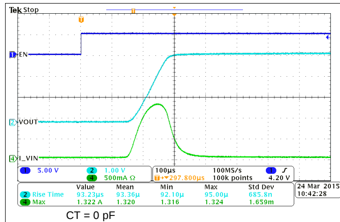
Figure 64. Inrush with CT = 0 pF
