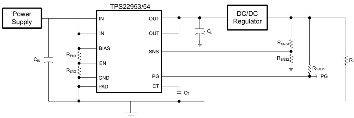
Figure 59. Monitoring a Downstream Voltage Schematic
