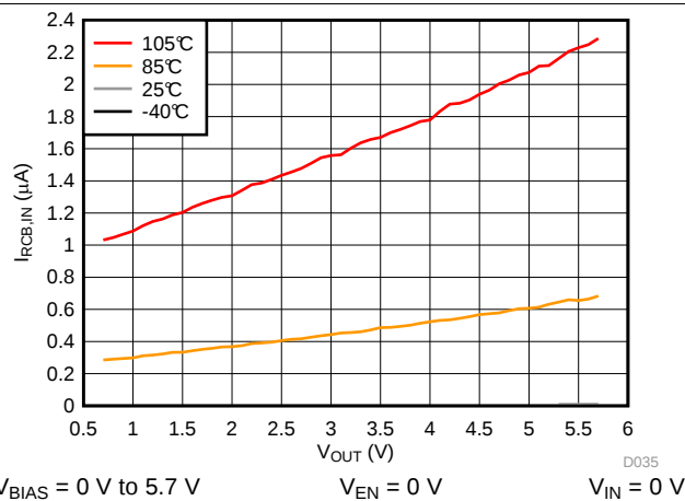
Figure 7. I_{RCB,IN} vs V_{OUT}
