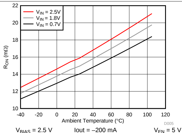
Figure 9. R_{ON} vs Temperature, V_{BIAS} = 2.5 V
