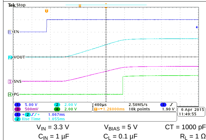
Figure 46. Turn On Waveform, Heavy Load
