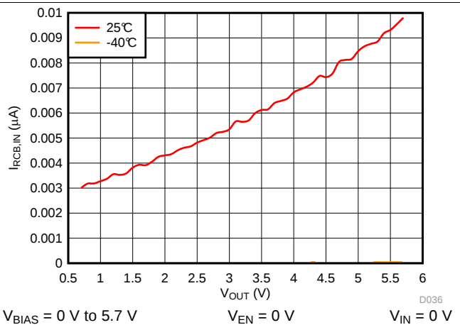
Figure 8. I_{RCB,IN} vs V_{OUT}
