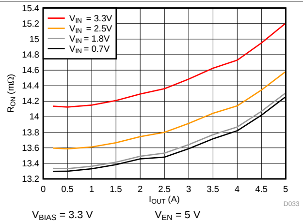
Figure 16. R_{ON} vs I_{OUT} , V_{BIAS} = 3.3\text{ V}
